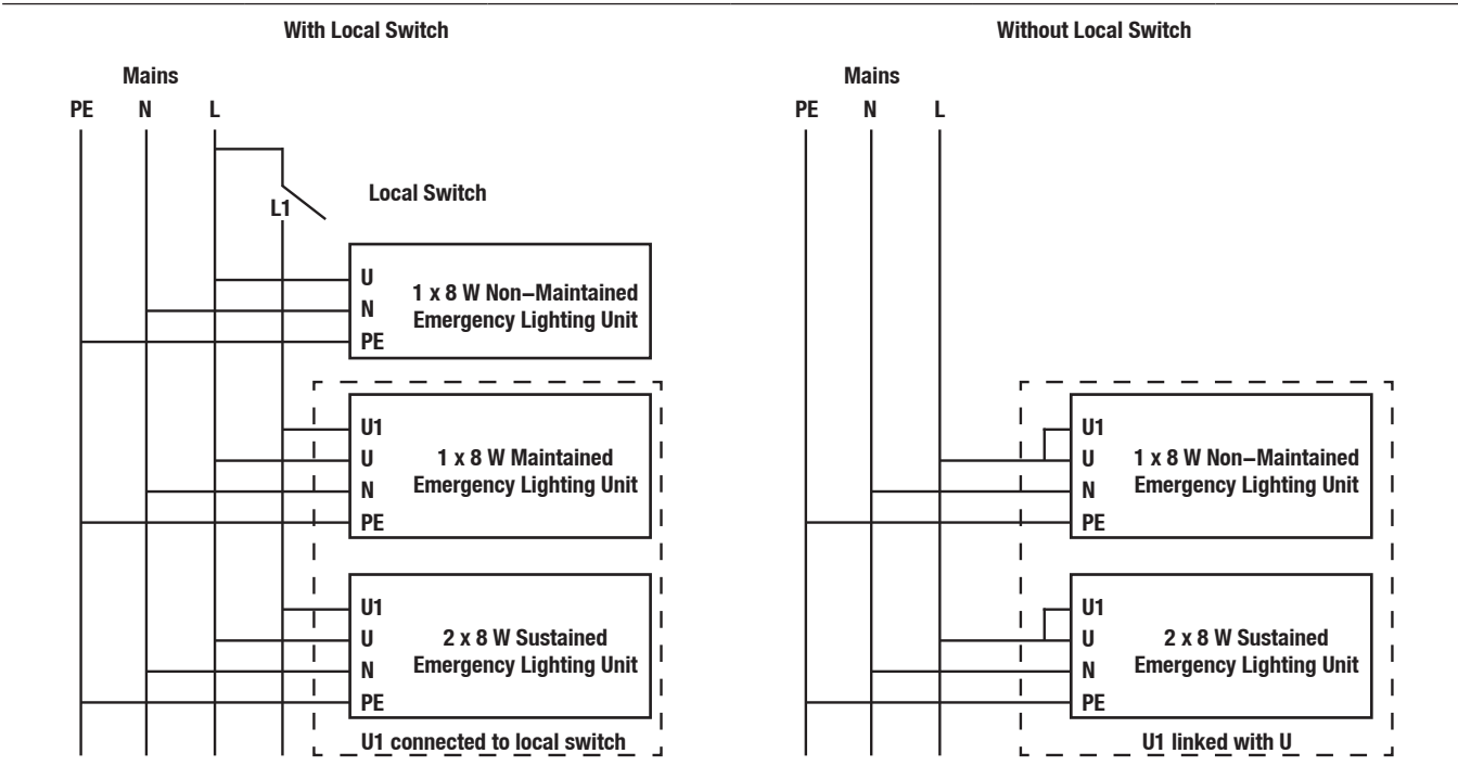
Emergency Function Diagram
