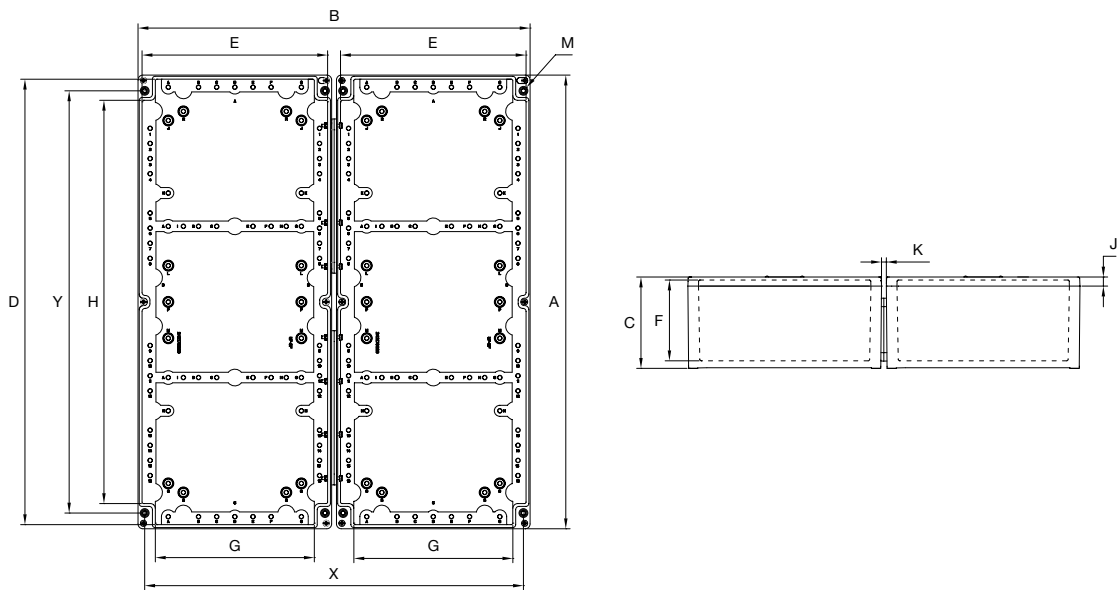
Dimensions in Millimeters (Inches) ①
